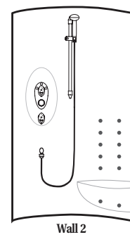
MAAX IES 3/4 with Body jets positioning
